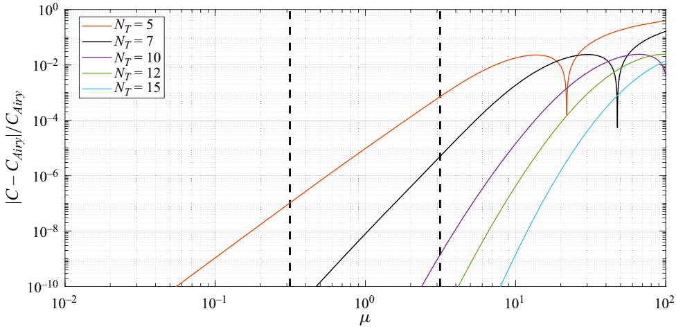
Figure 3. Relative error of the phase speed predicted by the linear wave version of the W3D model with different values of N_T in comparison with the analytical solution of Airy linear wave theory. Vertical dash lines denote the generally adopted shallow- and deep-water limits, \mu = kh = \pi/10 and \mu = \pi , respectively.
