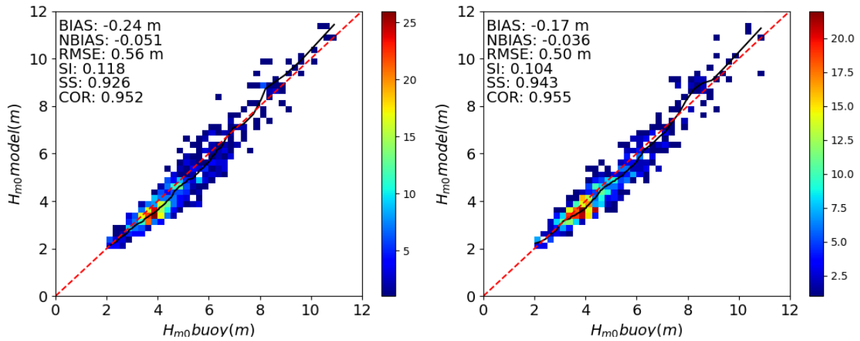
Fig. 9. Scatter plot and Q-Q plot of modelled versus measured H_{m0} domains at Belle-Ile buoy for ANEMOC-3 (left) and calibrated (right) configurations.
