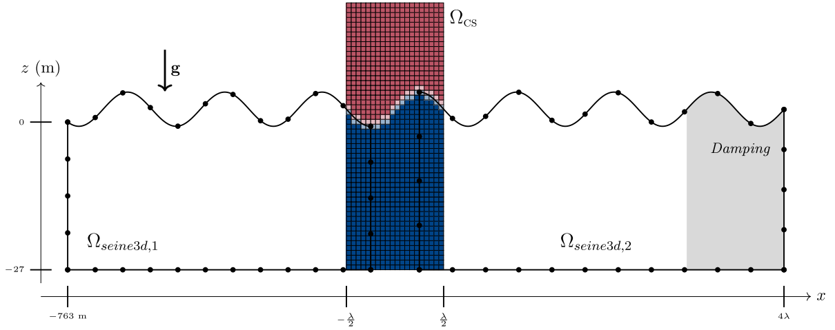
Fig. 7. Coupled domains for periodic wave simulations. Blue CS cells are cells filled with water, while red cells are full of air. Pale blue and pale red cells contain a mix of the two phases. CS mesh and seine3d boundary elements are drawn for illustrative purposes only. Horizontal proportions are realistic and correspond to the case of T = 15 s. The area in shaded gray represents the damping region in \Omega_{seine3d,2} , one wavelength long (given in Table 1).
