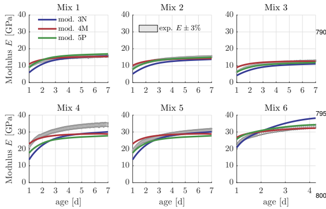
Figure 12: Model performance for early-age elastic modulus evolutions based on Mixes 1-6
