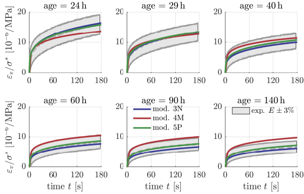
Figure 5: Model performance for Mix 1, cement paste w/c=0.42
