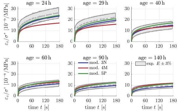
Figure 7: Model performance for Mix 3, cement paste w/c=0.50
