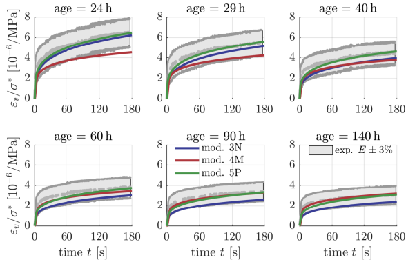
Figure 8: Model performance for Mix 4, mortar w/c=0.50
