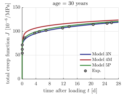
Figure 11: Model performance for long-term creep test at mature ages (Mix 7), cement paste w/c=0.50
