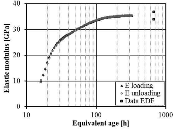
Figure 2: Evolution of loading and unloading moduli of VeRCoRs concrete (Mix 6), determined from hourly-repeated 5-min creep testing at early ages, and 28-days-stiffness values determined by EDF [17]
