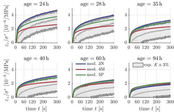
Figure 10: Model performance for Mix 6, concrete w/c=0.52
