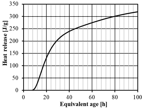
Figure 1: Calorimetry-based cumulative heat release Q for VeRCoRS concrete (Mix 6) as function of the age of the material
