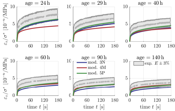
Figure 9: Model performance for Mix 5, concrete w/c=0.50
