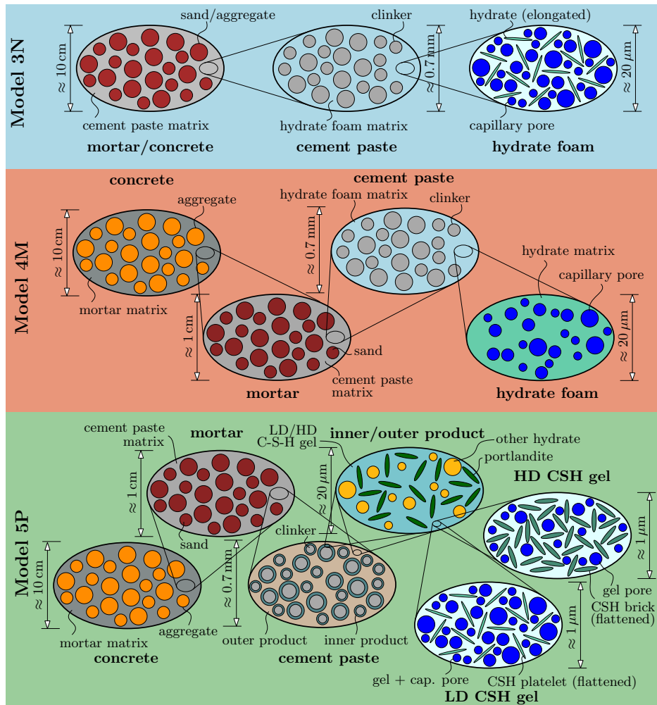
Figure 4: Material organograms representing the envisaged hierarchical organization of concrete: (a) Model 3N: 3-scale representation including needle-shaped hydrates after Pichler and Hellmich [5], Königsberger et al. [7]; (b) Model 4M: simplified 4-scale representation including a hydrate matrix after Honorio et al. [6]; (c) Model 5P: 5-scale representation including platelet-shaped hydrates, multi-hydrate extension of Sanahuja et al. [3, 37]; the two-dimensional sketches illustrate qualitative properties of three-dimensional representative volume elements
