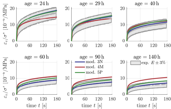
Figure 6: Model performance for Mix 2, cement paste w/c=0.45
