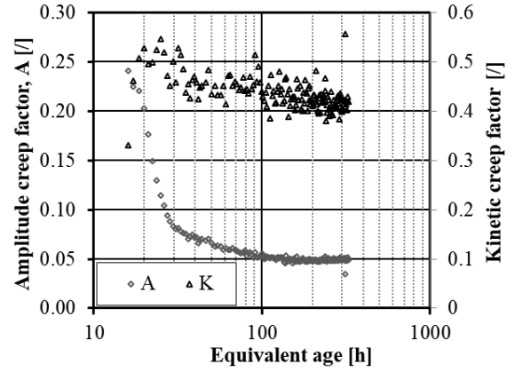
Figure 3: Evolution of the creep parameters A and K for VeRCoRs concrete (Mix 6), determined from hourly-repeated 5-min creep testing at early ages
