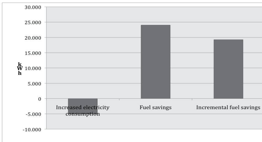
Figure 2. Increased electricity consumption and fuel savings.
