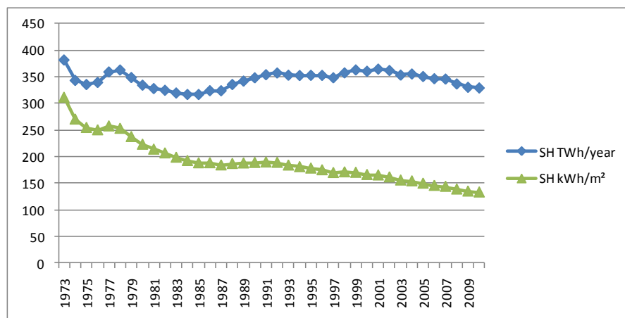
Figure 2. Evolution of total and unitary Space Heating (SH) consumption of PR stock (source: CEREN, climate adjusted final energy: TWh te /year and kWh te /[m 2 .year]).
