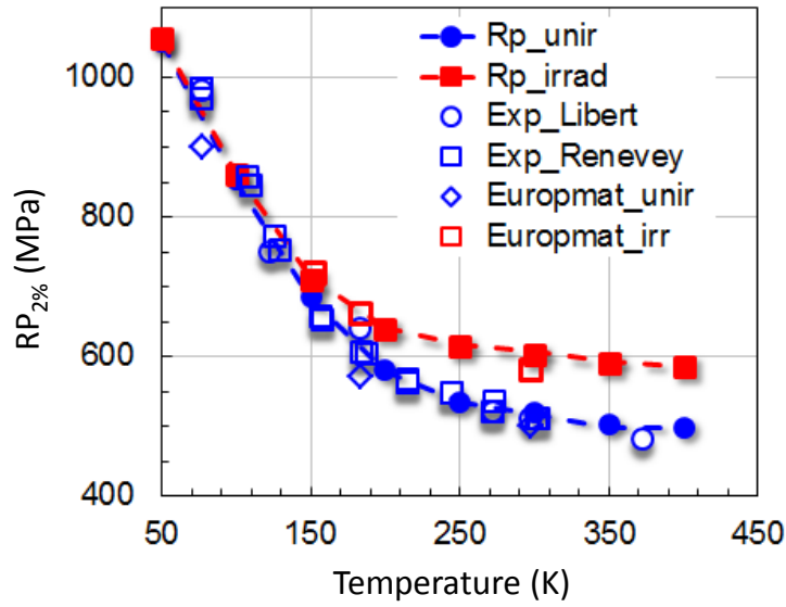
Figure 6: comparison between the BZ predictions (full symbols) and experimental values (open symbols) of the flow stress at 2% offset strain in RPV steels before (in blue) and after (in red) irradiation as a function of the simulation/experimental temperature of the tensile tests.
