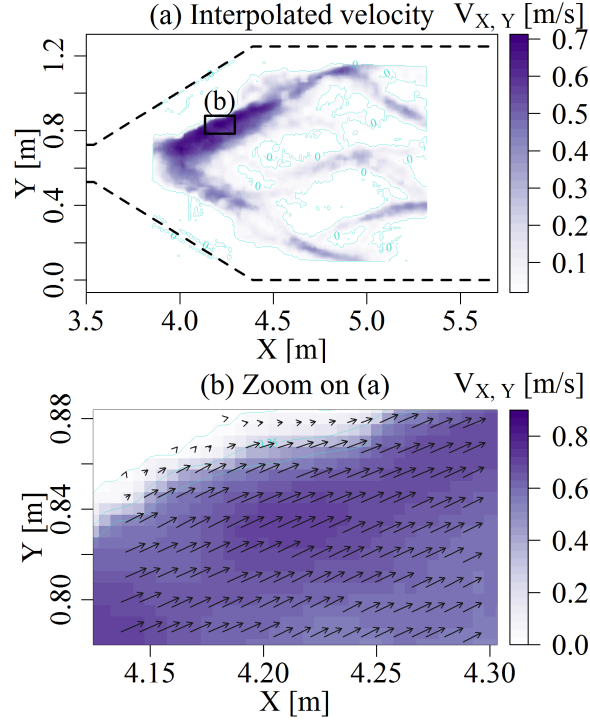
Figure 5: Surface velocities: a) Interpolated mean velocity V_{X,Y} on a regular grid ( \Delta X = \Delta Y = 5\text{mm} ), and b) zoom with both interpolated velocity field and LSPIV velocity vectors higher than 0.02 m/s (GSD2, QI=1.7 1/s, t=48 min)
