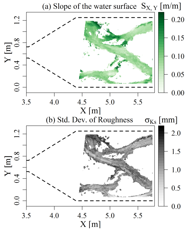
Figure 8: Friction law parameters: a) Slope of the water surface S_{X,Y} ; and b) Roughness standard deviation in the flow direction \sigma_{Ks_{X,Y}} (GSD2, Q_l=1.7 l/s, t=48 min). Note that since S_{X,Y} and \sigma_{Ks_{X,Y}} are computed along flow directions, they are not computed in dry areas (white areas in the figure) although these areas have absolute roughness and slope as seen on Figure 6
