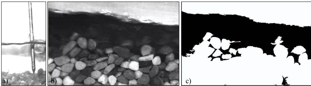
Figure 1: Side views of steep flows over a mobile bed composed of nearly uniform grains: a) illustration of the use of a point gauge: epistemic uncertainty related to the variable bed level and free surface, b) side view showing mobile grain clusters and perturbed free surface highlighting how uncertain the water depth measurement is, c) same image after threshold analysis showing the local variability of the water depth in bedload-laden flows
