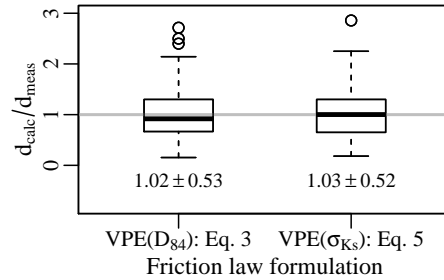
Figure 9: Statistical distribution of the ratio: computed water depth / measured water depth, water depth computed using the Ferguson (2007) form (VPE( D_{84} ): Eq. (3)) and the modified Ferguson form (VPE( \sigma_{Ks} ): Eq. (5)). Numbers below the boxes are mean values and standard deviations, upper circles are outliers higher than 1.5 the interquartile range.
