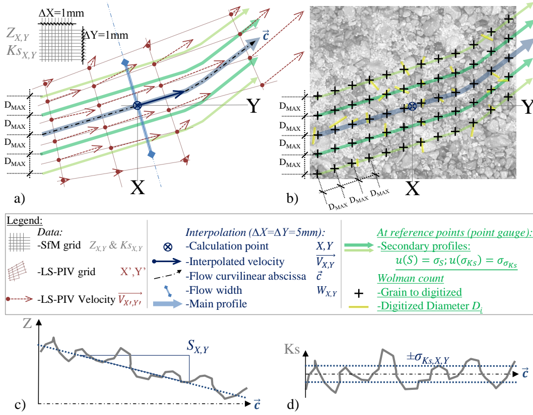
Figure 7: Sketch of the friction law parameters extraction algorithm: a) location of the flow profiles and curvilinear abscissa \bar{c} : parallel to the local velocity interpolated at point X,Y ; b) location of the Wolman count performed at reference points: precisely on the same main and secondary profiles; c) water surface slope S_{X,Y} extraction by a linear fit of Z_{X,Y} along \bar{c} ; and d) flow roughness \sigma_{Ks_{X,Y}} extraction: standard deviation of Ks_{X,Y} along \bar{c} . Parameters underlined in the legend are extracted only at reference points, while data and interpolation parameters are available at least on all of the LSPIV-measured area.
