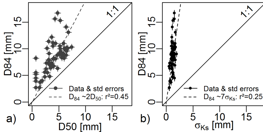
Figure 10: Statistical correlation between roughness proxies: a) D_{84} \approx 2D_{50} and b) D_{84} \approx 7\sigma_{Ks} .
