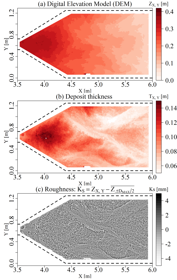
Figure 6: Bed topography data: a) Bed elevation Z_{X,Y} ; b) Deposit thickness T_{X,Y} ; and c) Surface roughness K_{S,X,Y} (GSD2, Q_1=2.2 l/s, t=25 min)
