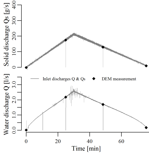
Figure 4: Typical boundary conditions: solid and water discharges at the inlet; black diamonds indicate time of LSPIV and SfM measurements; here the experiment was stopped twice, the data acquired are analyzed in subsequent figures (GSD2, peak water discharge: 2.7 l/s, peak solid discharge: 214 g/s, time to peak: 30 min).
