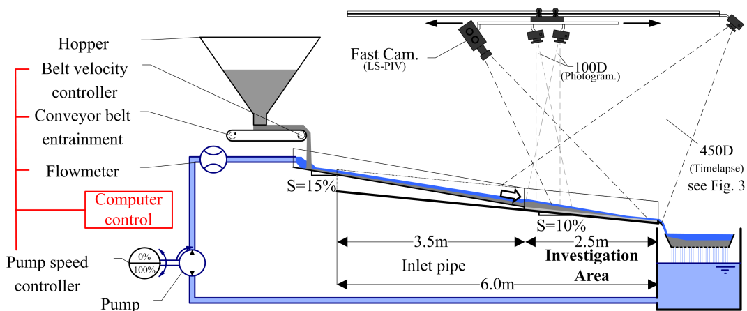
Figure 2: Experiment set-up : sediment-fed configuration and recirculation of water with four cameras for image acquisition
