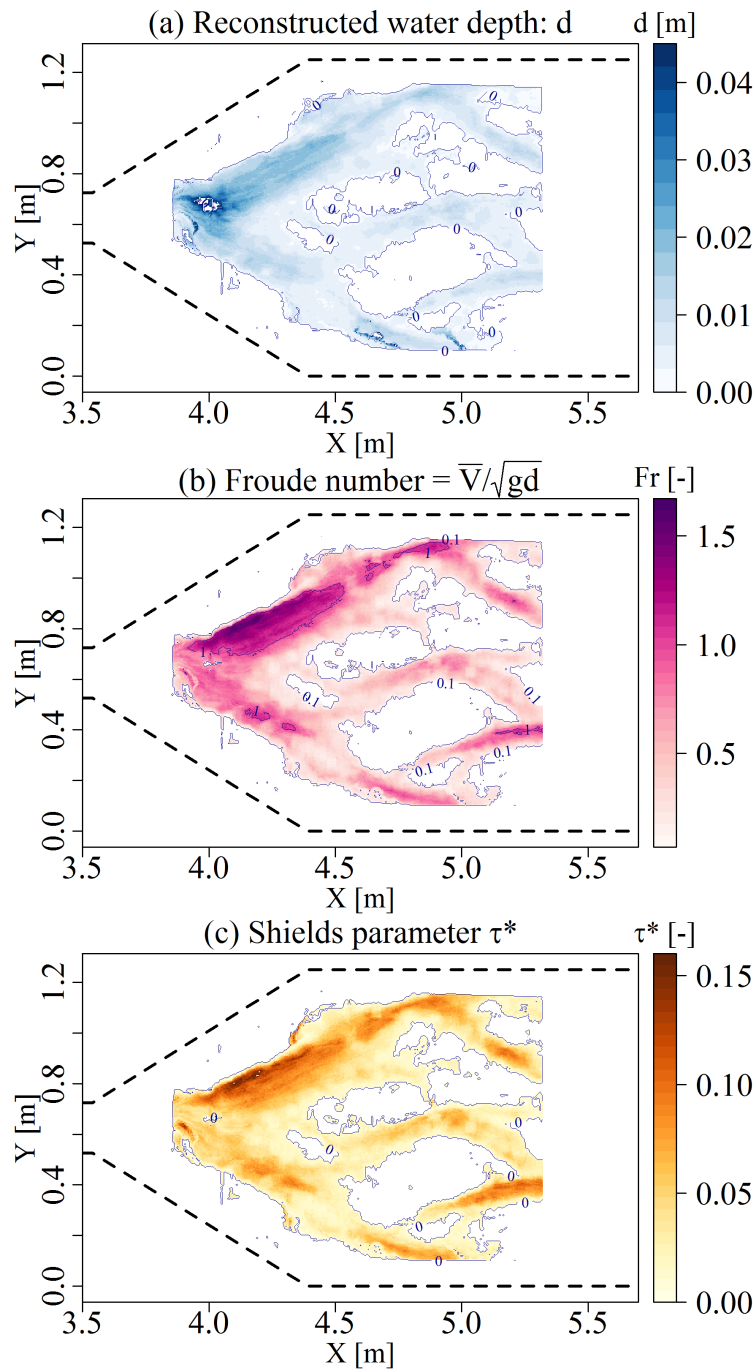
Figure 11: Maps of inversely computed flow properties: a) water depth d , b) Froude number V/\sqrt{gd} and, c) Shields parameter \approx Sd/[(s - 1)7\sigma_{K_s}] (GSD2, Ql=2.2 l/s, t=25 min)
