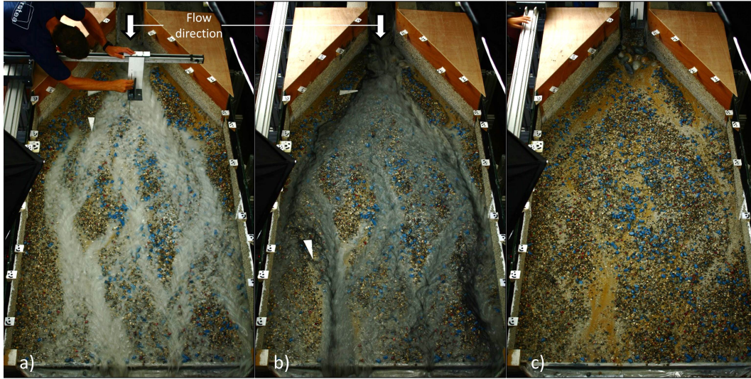
Figure 3: Images of the investigation area: a) flow depth local measurement with a point gauge, a few seconds later, b) flow seeded with charcoal powder clouds during the LSPIV image capture, immediately followed by c) stopping of the experiment and drained-bed image capture for SfM photogrammetry acquisition. Only measures with negligible morphological changes between LSPIV and SfM acquisitions were used in flow reconstruction. The white triangle marks the gauge measure abscissa. Note that the flow may touch one side wall but remains an unconfined flow because the other bank can erode or aggrade to adjust the channel width.
